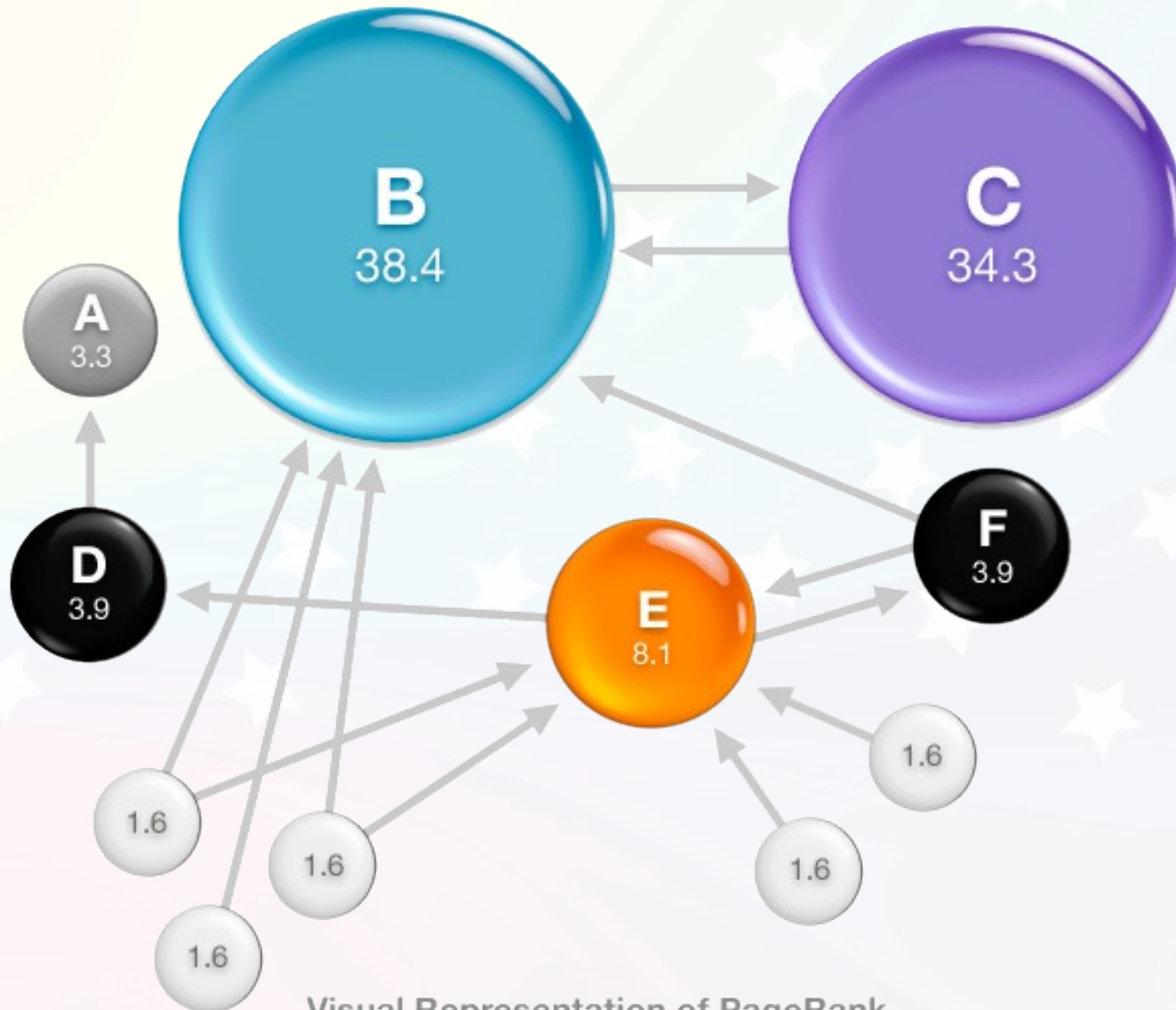
Visual Representation of PageRank
